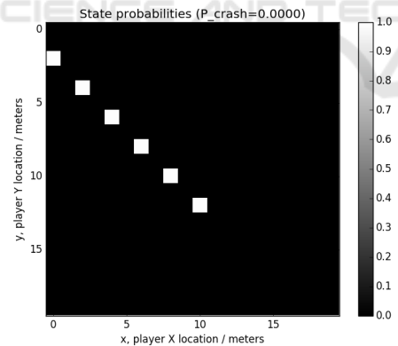
Figure 8: Sequential chicken state probabilities, from asymmetric start (12,10).
