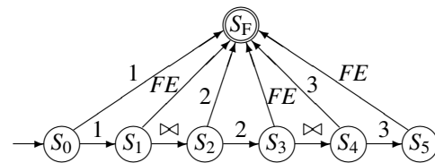
Figure 1: NFA for the winning pattern sequel.
