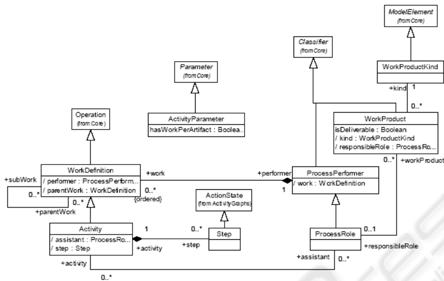
Figure 2: Process_Structure package of SPEM.
