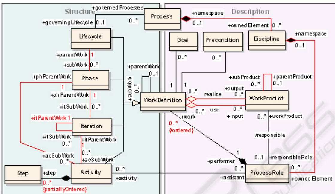
Figure 3: Extract of our specialization of SPEM metamodel.
