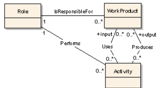
Figure 1: SPEM conceptual model.
