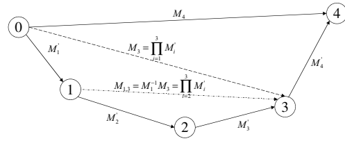
Figure 3: The integration of single-step estimations can be obtained by just multiplying the individual motion matrices. Every circle denotes the state (position and orientation) of the camera between time t_0 and time t_4 . Vectors indicate motion in 3D-space.
