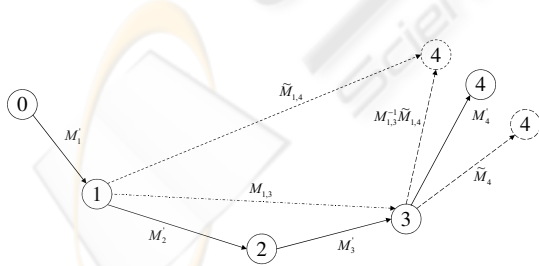
Figure 4: multi-frame approach. Circles represent the position and orientation of the camera. Vectors indicate motion in 3D-space. \tilde{M}_4 (single step estimation) and M_{1,3}^{-1} \tilde{M}_{1,4} (multi-step estimation) are interpolated in order to obtain the final estimation M'_4 .
