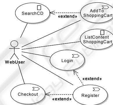
(a) Use case model.
