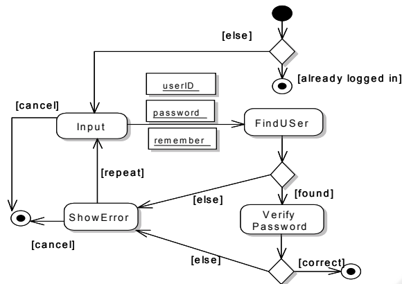
Figure 3: Activity diagram for the Login use case (UWE).
