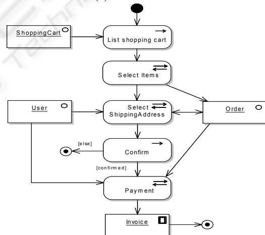
(b) UML activity diagram.
