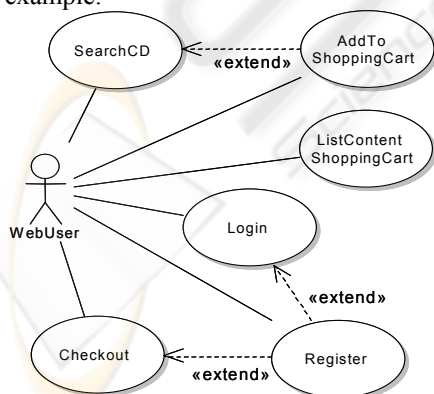
Figure 1: UML use case diagram for the CD e-shop.
