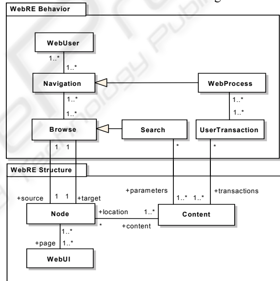
Figure 4: Metamodel for Web Requirements Engineering (WebRE).
