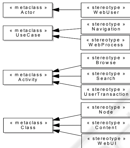
Figure 5: Modeling Elements of UML Profile for Web Requirements Engineering (WebRE).
