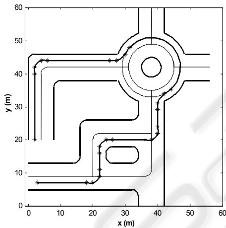
Figure 8: Generated trajectory using trigonometric splines.
