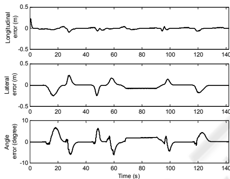
Figure 14: Angle, longitudinal and lateral tracking errors, using a Kanayama controller and the vehicle kinematics model to follow clothoid curves planned trajectory.
