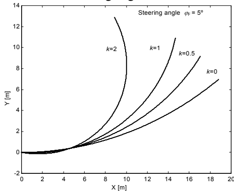
Figure 4: Car-like vehicle trajectories, using the same front wheel steering angle \varphi_F = 5^\circ and different values of the rear steering angle, given by the coefficient k .
