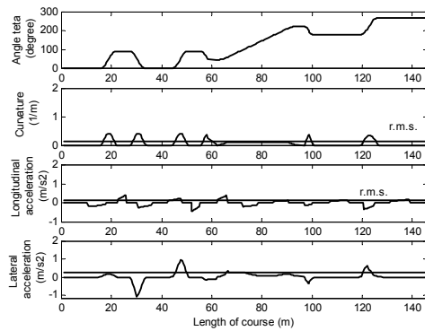
Figure 13: Orientation angle \theta , curvature, longitudinal and lateral acceleration behaviour along the course for the given reference speed profile, using clothoid curves trajectory planning.
