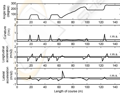
Figure 9: Orientation angle \theta , curvature, longitudinal and lateral acceleration behaviour along the course for the
