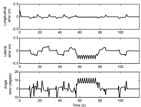
Figure 12: Angle, longitudinal and lateral tracking errors, using a Kanayama controller and the vehicle kinematics model to follow cubic trigonometric planned trajectory.
