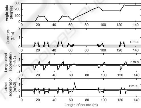
Figure 11: Orientation angle \theta , curvature, longitudinal and lateral acceleration behaviour along the course for the given reference velocity vector, using trigonometric splines trajectory planning.
