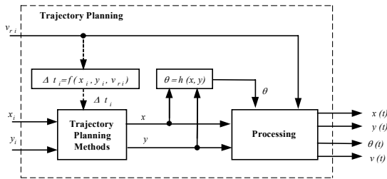
Figure 6: Trajectory planning module.
