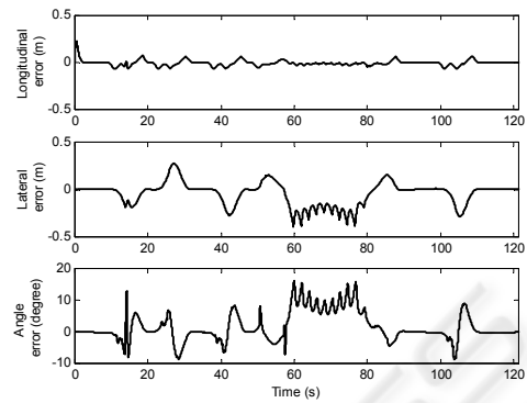
Figure 10: Angle, longitudinal and lateral tracking errors, using a Kanayama controller and the vehicle kinematics model to follow cubic splines planned trajectory.
