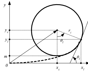
Figure 5: Transition from a straight line to a circumference arc using a clothoid curve. m represents the distance between the straight line and the circumference.
