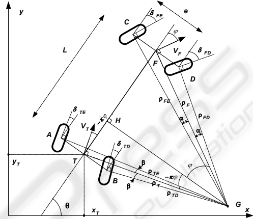
Figure 3: Kinematics model of a 4-wheel car-like vehicle with front and rear steering capability.
