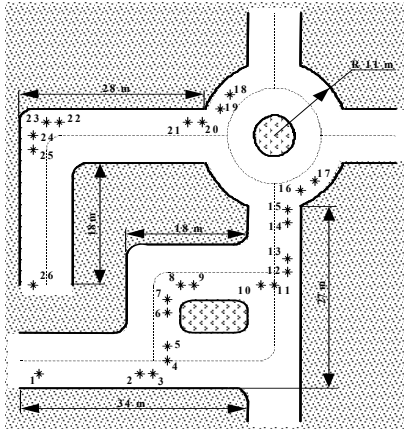
Figure 1: Urban road way with very close corners, a roundabout, and waypoints defined by stars.
