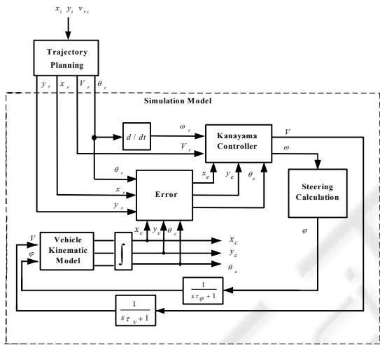
Figure 7: Simulation model block diagram: trajectory planning and trajectory-tracking modules.
