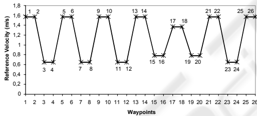
Figure 2: Speed profile defined by speed values at the waypoints specified in Fig. 1: v_{ri}, i = 1, 2, \dots, 26 .
