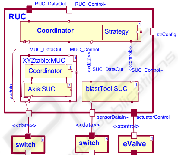
Figure 5: Components of CCAS in XYZ table Control Unit.
