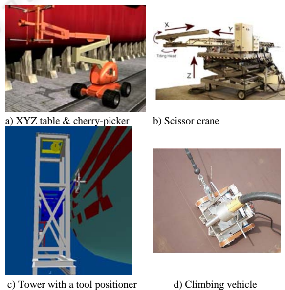
Figure 1: Different solutions for grit blasting
