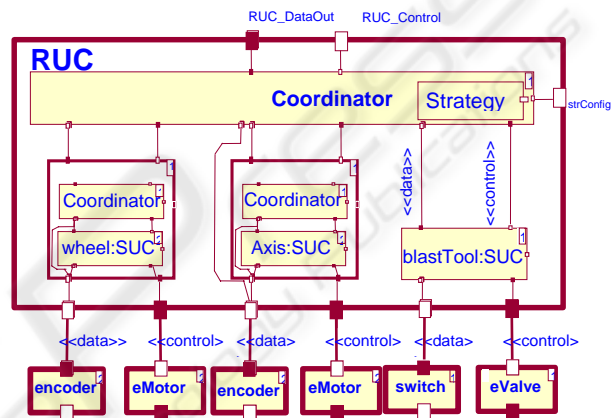
Figure 7: Components of CCAS in climbing vehicle
