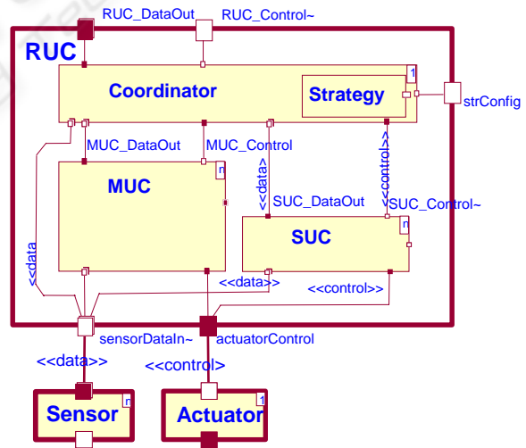
Figure 4: RUC: Robot Unit Controller.
