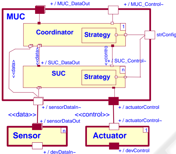
Figure 3: MUC and SUC. 1 actuator - N sensors
