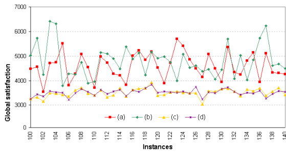
Figure 5: Close up on global satisfaction between methods: (a) GS man-optimal (b) GS woman-optimal (c) Zigzag man-optimal and (d) Zigzag woman-optimal
